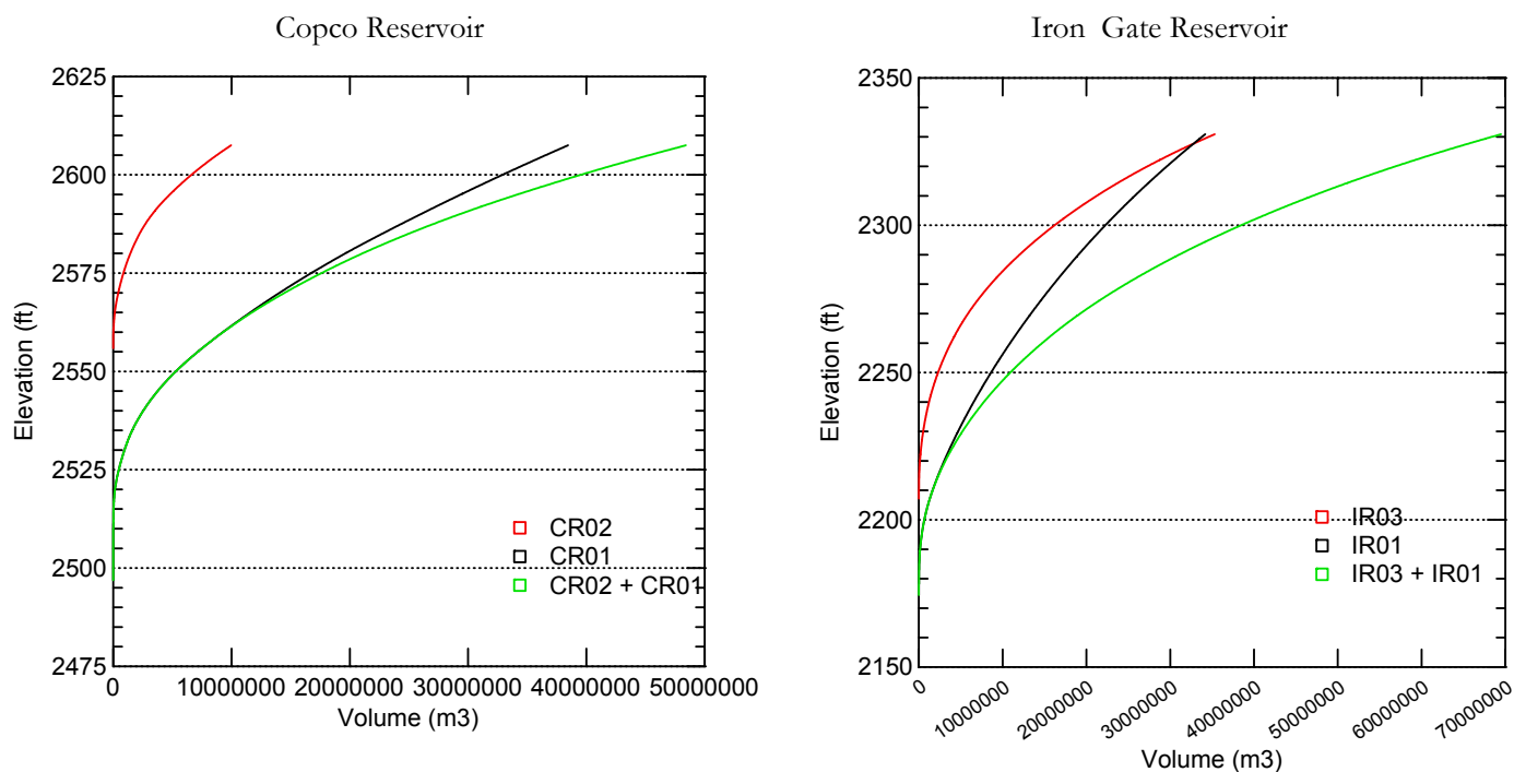
Fig. 6. Water surface elevation-volume curves for Copco and Iron Gate Reservoirs as a whole, and for the eastern and western portion of each reservoir separately.
