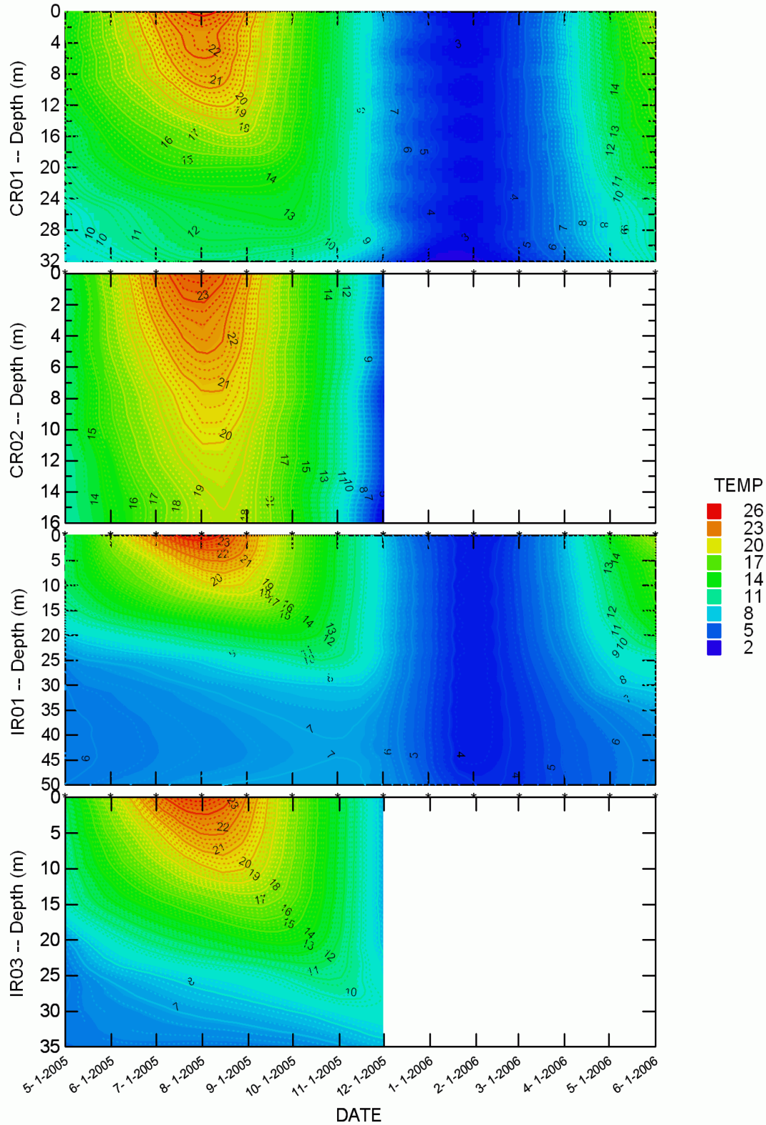
Fig. 8. Depth-time distributions of isotherms of temperature ( ^{\circ}\text{C} ) at stations in Copco and Iron Gate Reservoir, May 2005-May 2006.
