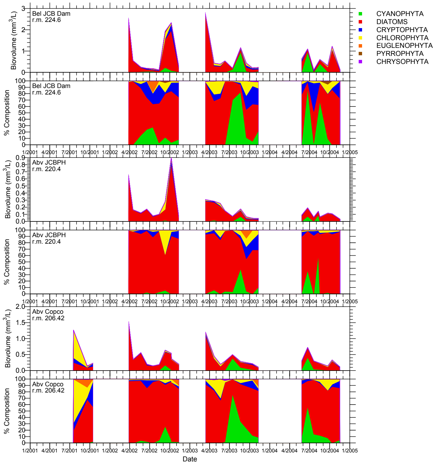
Figure 9. Biovolume and percent biovolume of major taxonomic groups of phytoplankton for surface samples collected in the years 2001-2004. Sites are listed in downstream order: Below J.C. Boyle Dam, Above J.C. Boyle Powerhouse, and Above Copco Reservoir.
