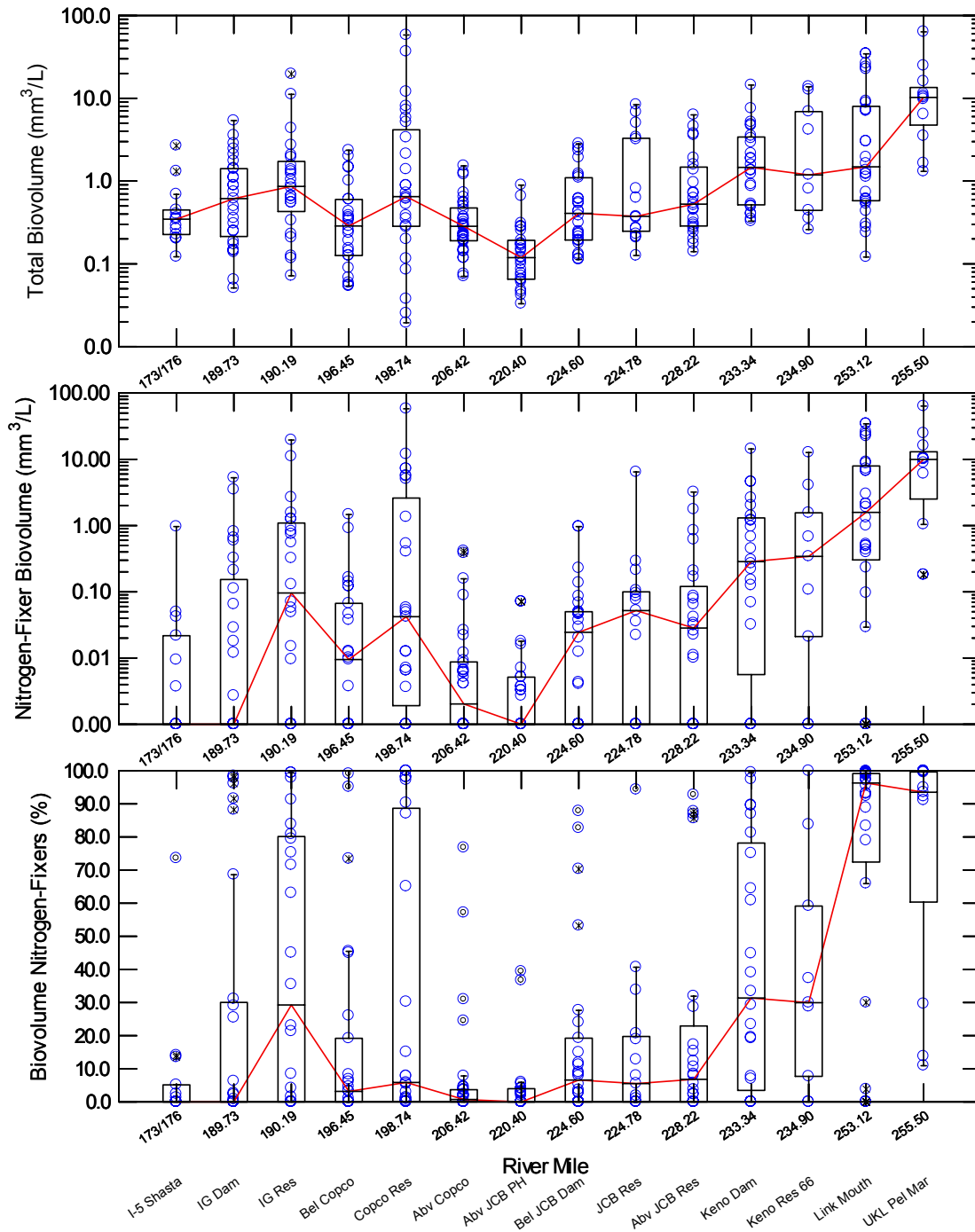
Figure 3. Total phytoplankton biovolume (top panel), total biovolume of nitrogen-fixing species (middle panel), and percent biovolume of nitrogen fixing species (bottom panel) of surface samples at major Klamath River sampling sites for the years 2001-2004, all months. The line inside each box is the median and the edges of each box are the 25 th and 75 th percentiles. The whiskers represent data points beyond 1.5 times the interquartile (75 th -25 th ) range, while individual points shown in black are outliers.
