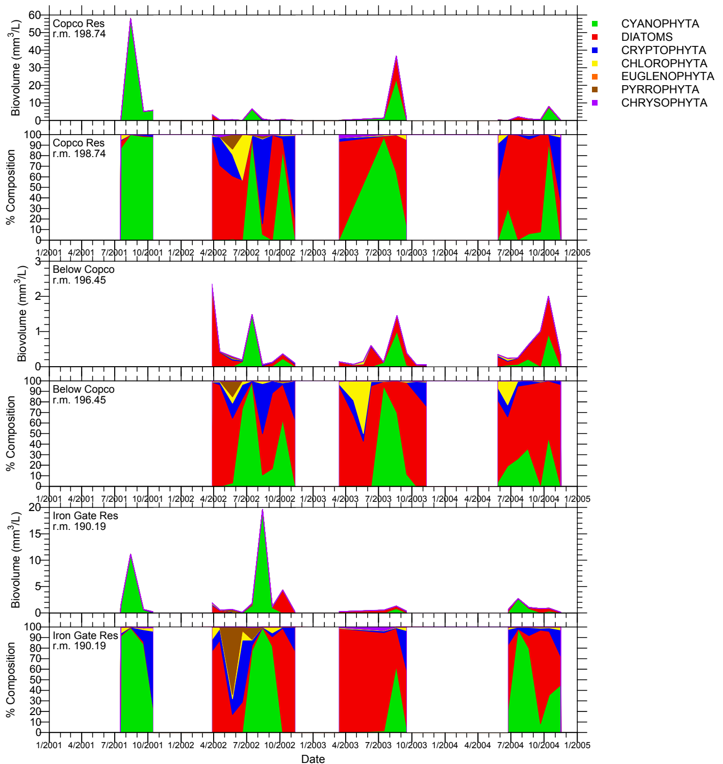
Figure 10. Biovolume and percent biovolume of major taxonomic groups of phytoplankton for surface samples collected in the years 2001-2004. Sites are listed in downstream order: Copco Reservoir, Below Copco Dam, and Iron Gate Reservoir.
