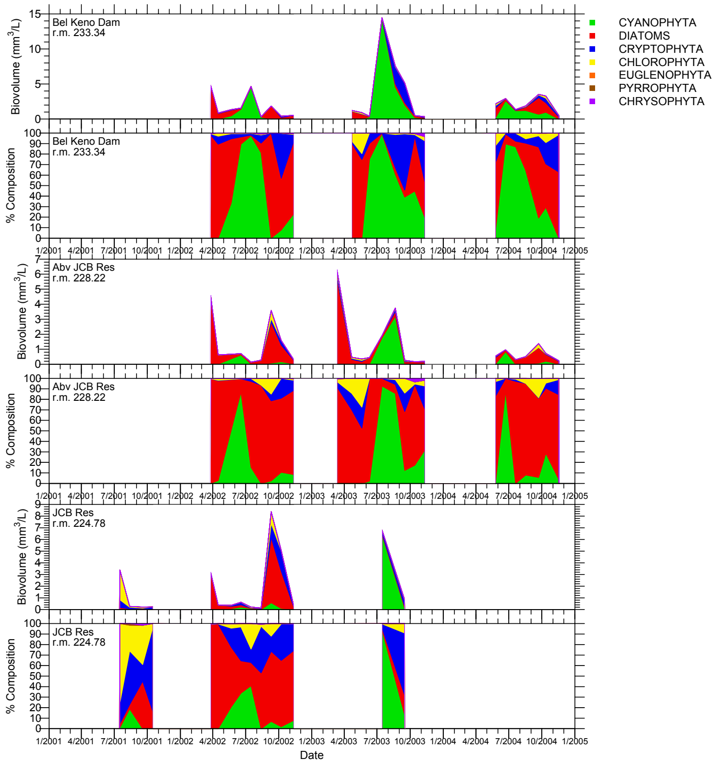
Figure 8. Biovolume and percent biovolume of major taxonomic groups of phytoplankton for surface samples collected in the years 2001-2004. Sites are listed in downstream order: Keno Dam, Above J.C. Boyle Reservoir, and J.C. Boyle Reservoir.
