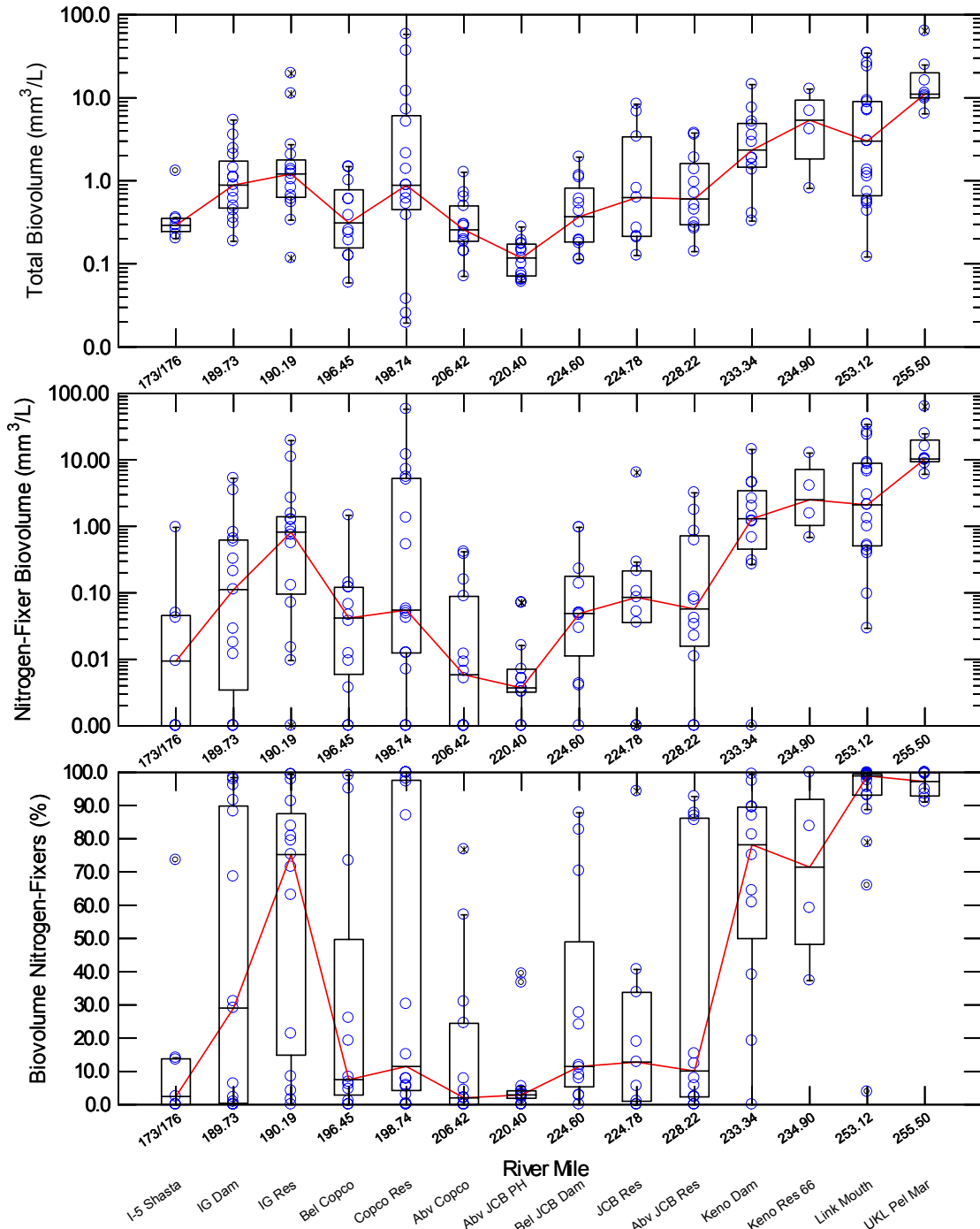
Figure 4. Total phytoplankton biovolume (top panel), total biovolume of nitrogen-fixing species (middle panel), and percent biovolume of nitrogen fixing species (bottom panel) of surface samples at major Klamath River sampling sites for the years 2001-2004, June 1- September 30.
