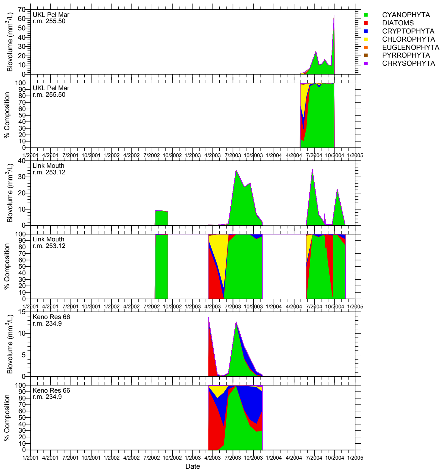
Figure 7. Biovolume and percent biovolume of major taxonomic groups of phytoplankton for surface samples collected in the years 2001-2004. Sites are listed in downstream order: Upper Klamath Lake at Pelican Marina, Link River at its mouth, and Keno Reservoir at the Highway 66 Bridge.
