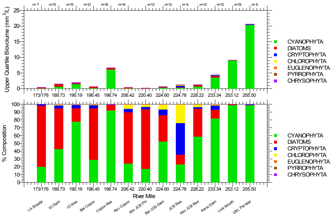
Figure 6. Median and upper quartile biovolume and percent composition of major phytoplankton taxonomic groups for surface samples collected June 1 – September 30, 2001-2004.
