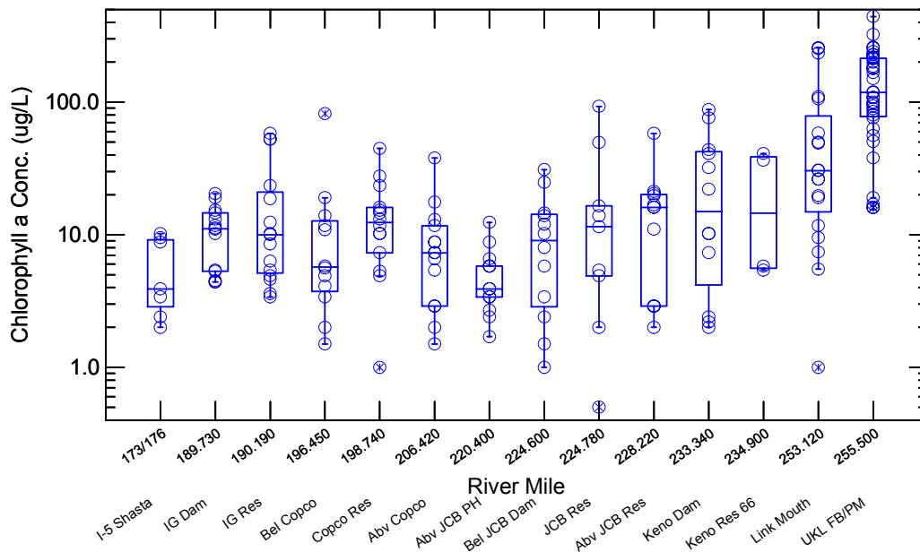
Figure 5. Chlorophyll a concentrations at Klamath River sites for all dates (top panel) and June-September (bottom panel), 2001-2004. Data are from samples collected by PacifiCorp and the Klamath Tribes.
