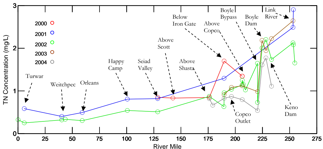
Figure 4. Longitudinal profile of mean summer (June 1 – August 31) total nitrogen concentrations in Klamath River mainstem sites for the year 2000-2004 (reservoirs excluded). Sites with less than three measurements in a summer were excluded from this graph. It is important to note that this graph, originally in Kier Associates (2005), summarizes data from a wide range of agencies,
