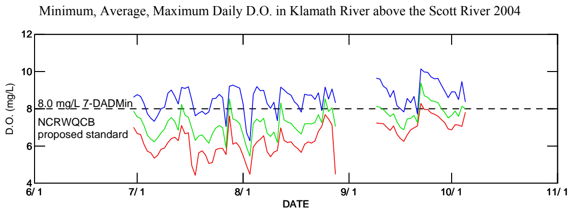
Figure 10. This chart shows minimum (red) , average (green) and maximum (blue) D.O. values for the Klamath River above the Scott River (RM 142.61) with a reference value showing the NCRWQCB (2006) proposed year-round standard that the seven-day moving average of the daily minimum D.O. should be 8 mg/L or greater. The proposed standard during spawning is that the seven-day moving average of the daily minimum concentrations should be at least 11.0 mg/L in the water column. Data are from the USFWS, Karuk Tribe, Yurok Tribe and USGS.
