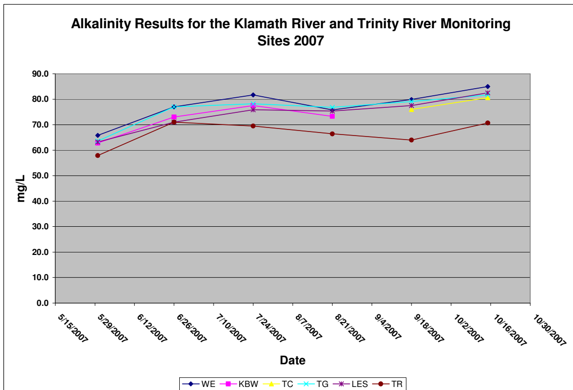
Figure 9. Alkalinity Results 2007
