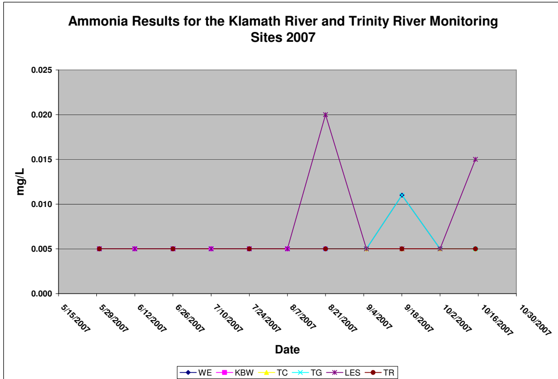
Figure 6. Ammonia Results 2007
