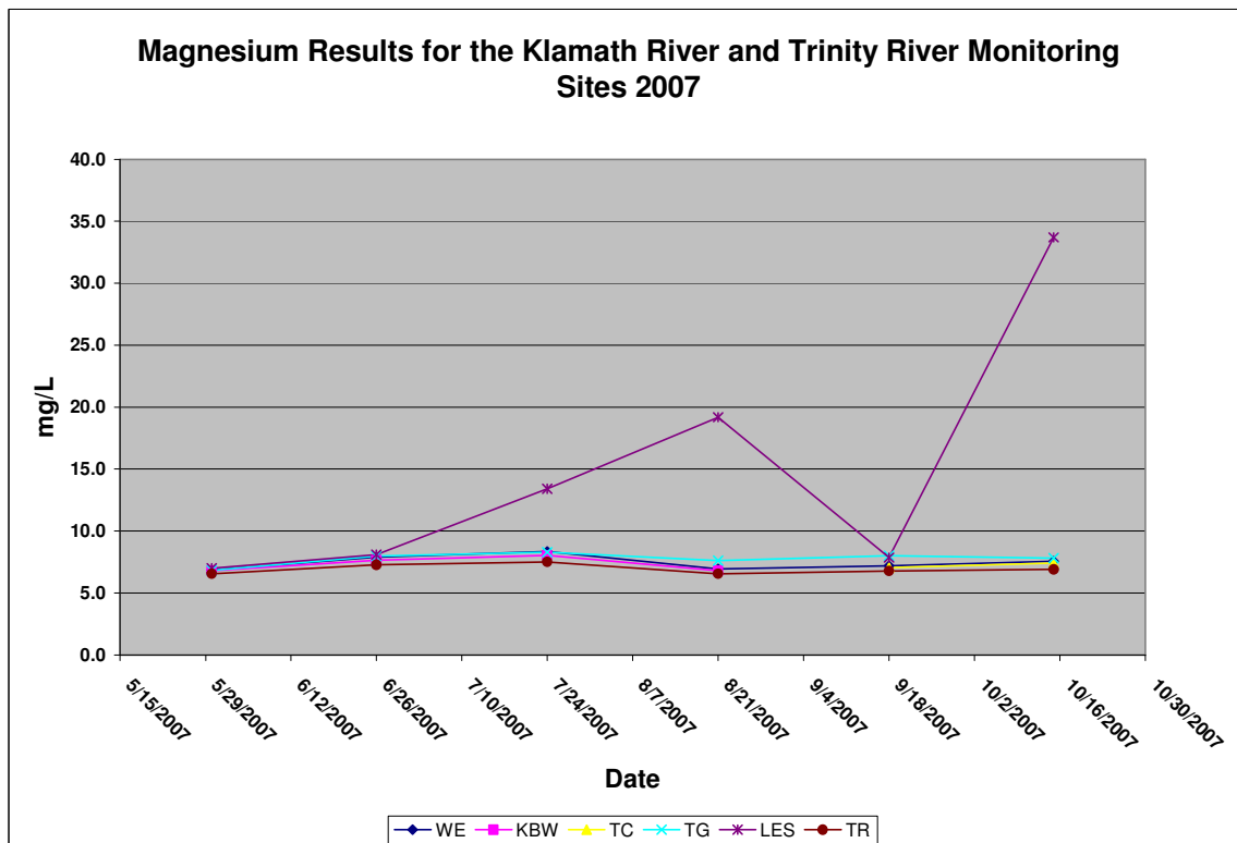
Figure 13. Magnesium Results 2007
