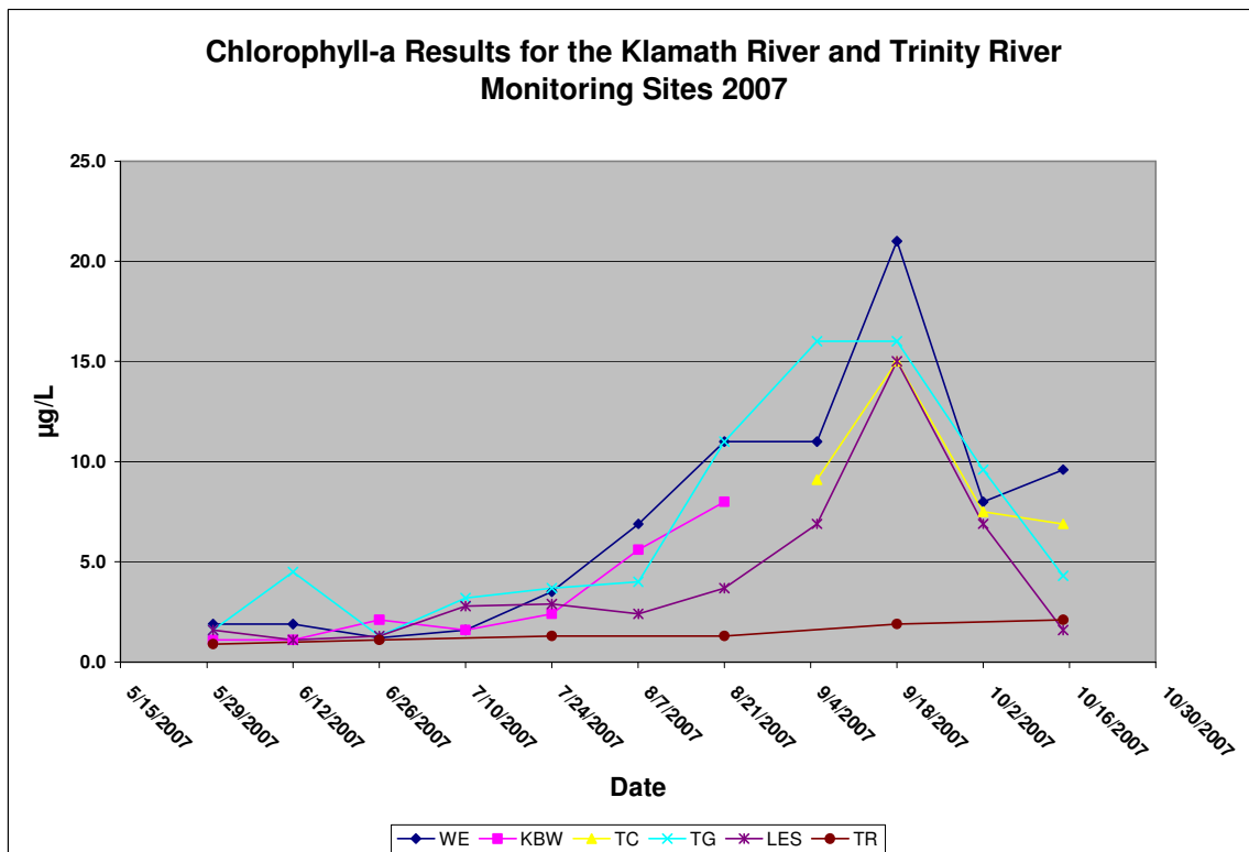
Figure 11. Chlorophyll-a Results 2007
