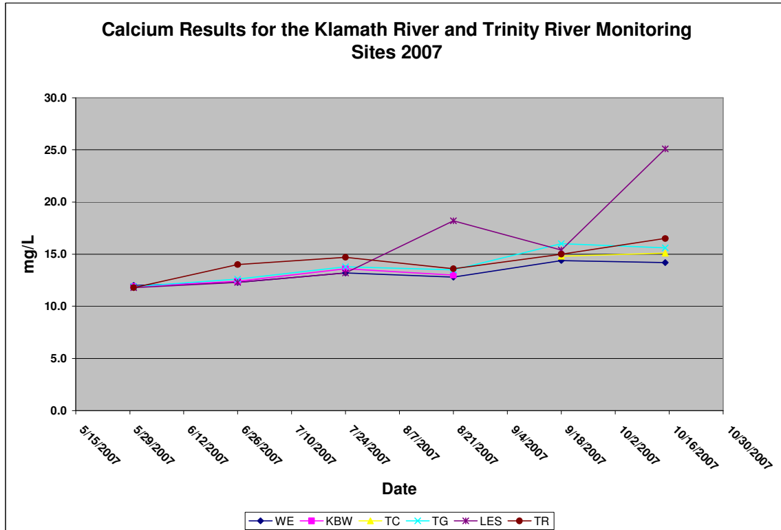
Figure 10. Calcium Results 2007
