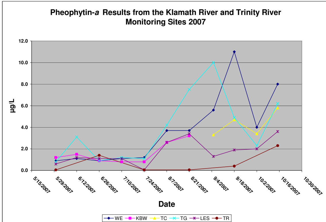
Figure 12. Pheophytin-a Results 2007
